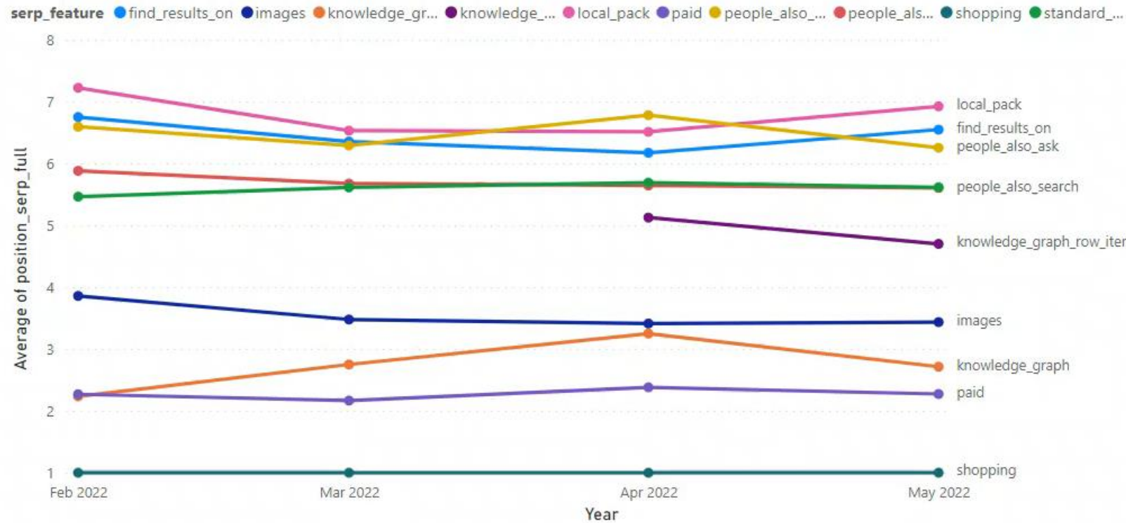
Average of position_serp_full by Year, Month and serp_feature
