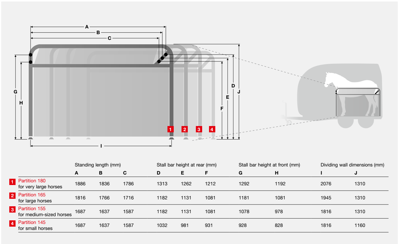
Comfortable transport for horses of all sizes with the dividing wall concept. On request you can equip your Neo with a dividing wall that perfectly fits your horse.
